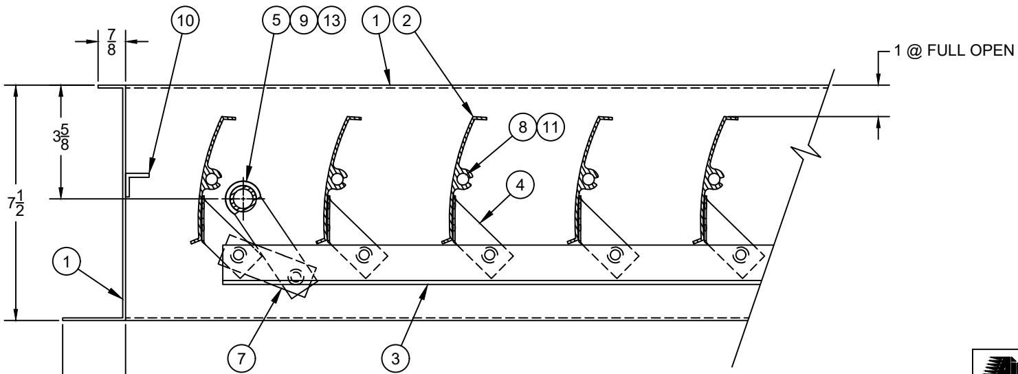
LOUVER @ FULL OPEN
